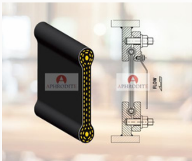
Dog Bone / Belt type Expansion Joints
